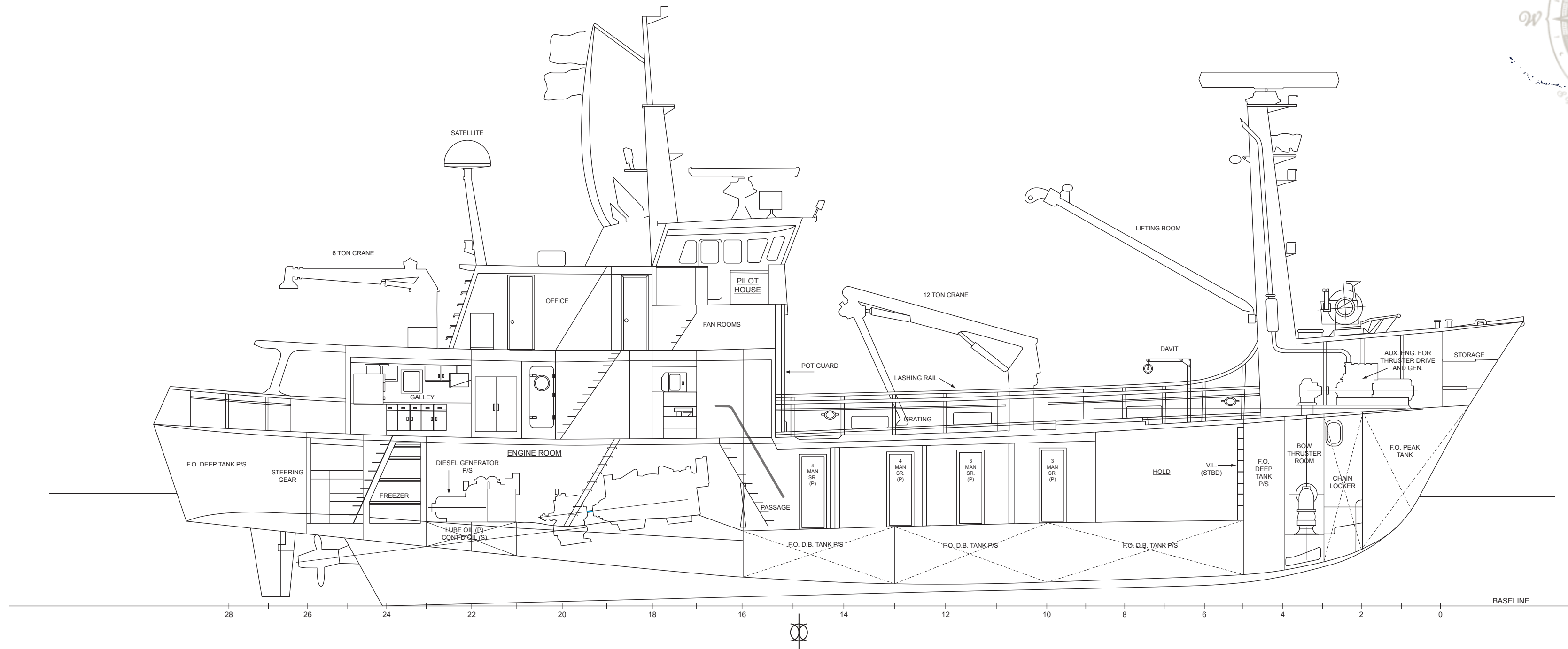
INBOARD ARRANGEMENT PROFILE
